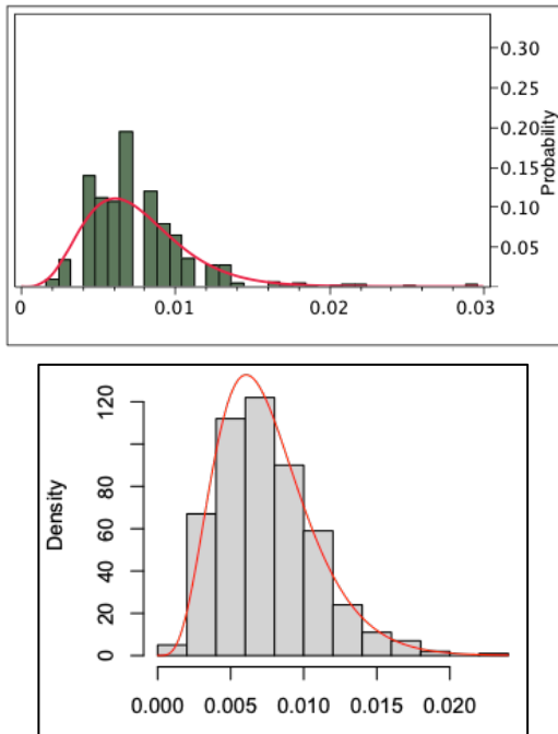
Figure A1. (upper) Histogram of actual spectral width values in Hz over a 21 km line-of-sight path from N6GN to N6GN/K with identical GPSDO master oscillators at the transmitter and receiver with a best-fit Gamma distribution. (lower) A synthesised histogram of a Gamma distribution of 500 values with the same Scale and Shape parameters as the observations.
