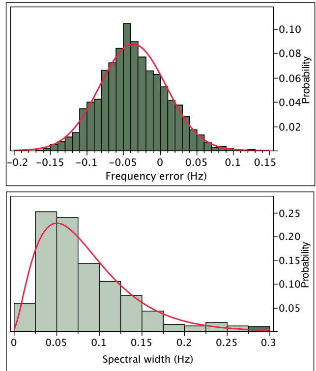
Figure 7. Two measures of short-term frequency variation in two KiwiSDRs. Upper: Histogram and fitted Gaussian distribution at G3ZIL of frequency error at 10 MHz at one-second intervals. Lower: Spectral width from jt9 at KPH from FST4W-120 GPSDO transmissions from K6PZB over a 38 km path.
